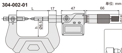
304-002-01
