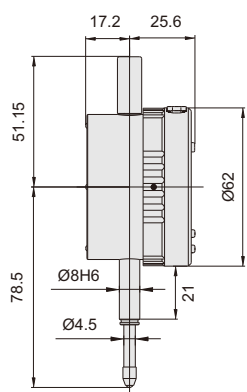
量程:0-12.7mm
