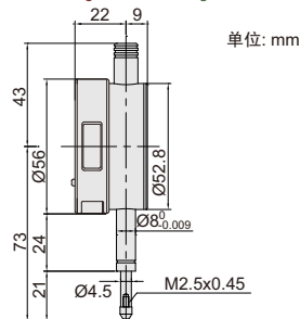
量程: 0-12.7mm
