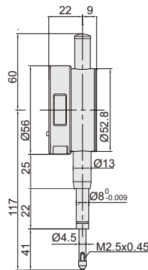
量程: 0-25.4mm
