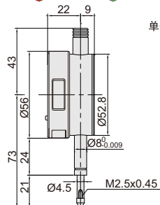
量程: 0-12.7mm
