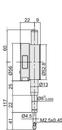
量程: 0-25.4mm
